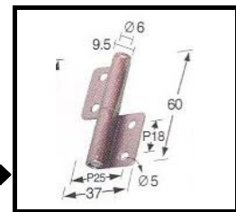
60# -2-4 STAINLESS STEEL DOOR HINGE
