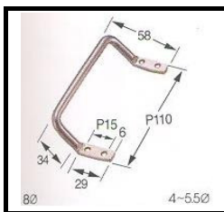
A-42-F STEEL ROUND BAR DRAWER PULL
