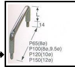
A-42-B STEEL ROUND BAR DRAWER PULL
