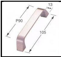
A-303 ZINC ALLOY DRAWER PULL
