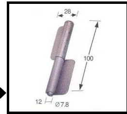
100# -2 STAINLESS STEEL DOOR HINGE
