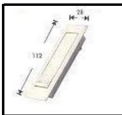
A-240-2E FLUSH HANDLE W/O KEY
